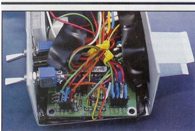
Photo C-Interior view of the "Freakin' Beacon" interface board, completed and installed. The electrical tape is to provide insulation for the transmitter board, which will be installed (upside down) above the interface circuitry.
